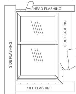
FIG.3, EXTERIOR VIEW
